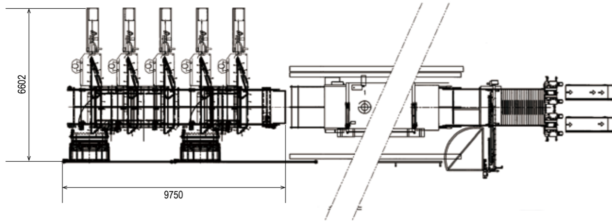
5 units of HITEC linkers set to 1 production line of continuous smoke house
